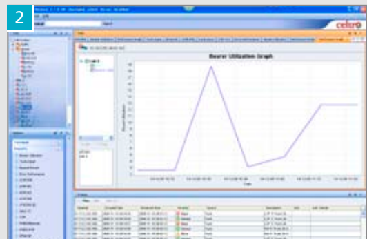
DMSView: Bearer Utilization Report
